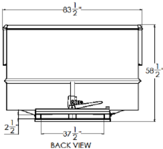
RUGGED 3T-3/16-1080
