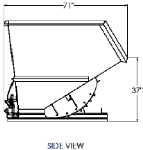
RUGGED 3T-3/16-1080
