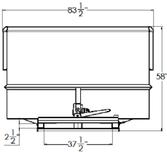
BACK VIEW
