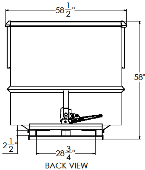
DURABLE 2T-10-680
