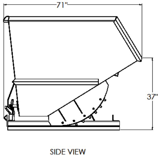
DURABLE 2T-10-680
