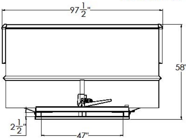
BACK VIEW
